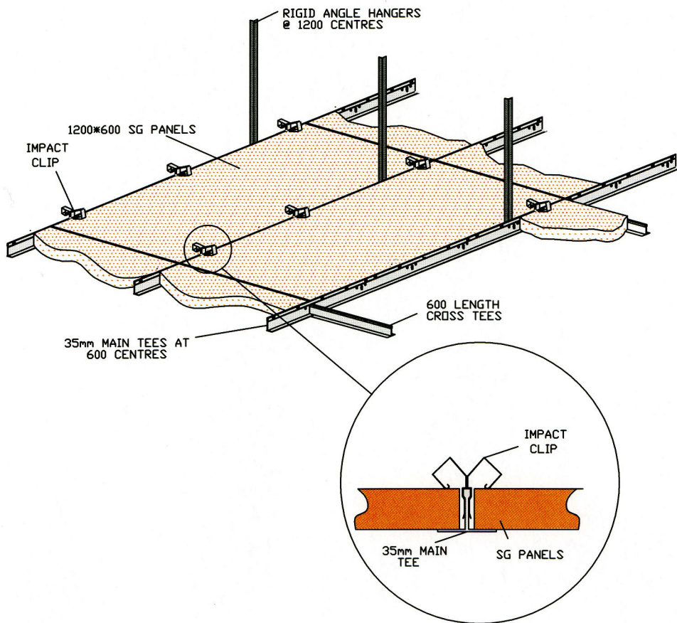
ALTERNATIVE INSTALLATION WITH IMPACT CLIPS
